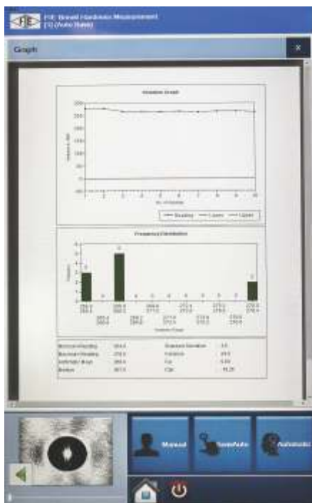
Statistics
