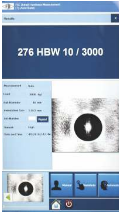
Result Window
