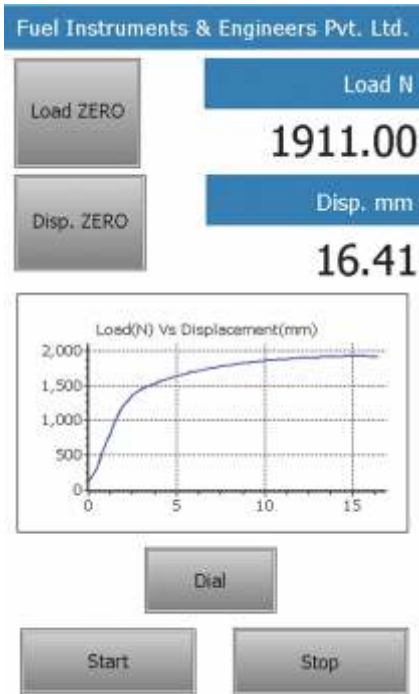
Real time Graph with load & displacement
